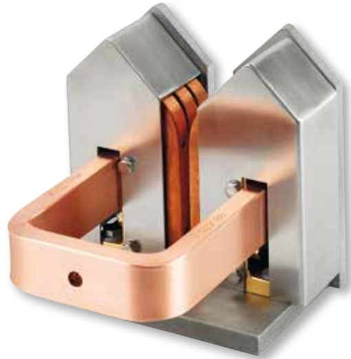
Contact saddle in special design with current feed through a bracket
