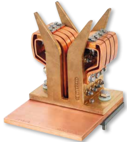
Finger contact saddle ready for installation with substructure
